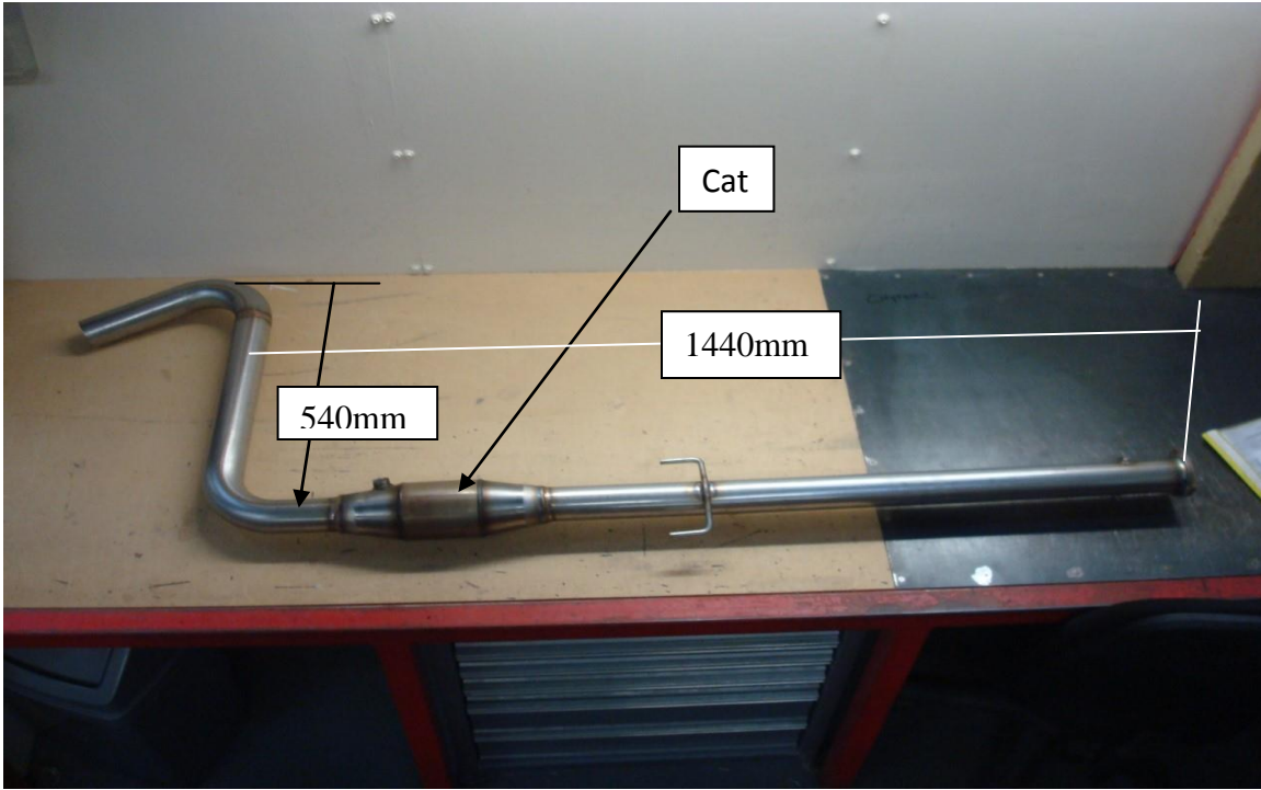
Fig 2 Centre Section. (material:- mild steel or stainless steel)
