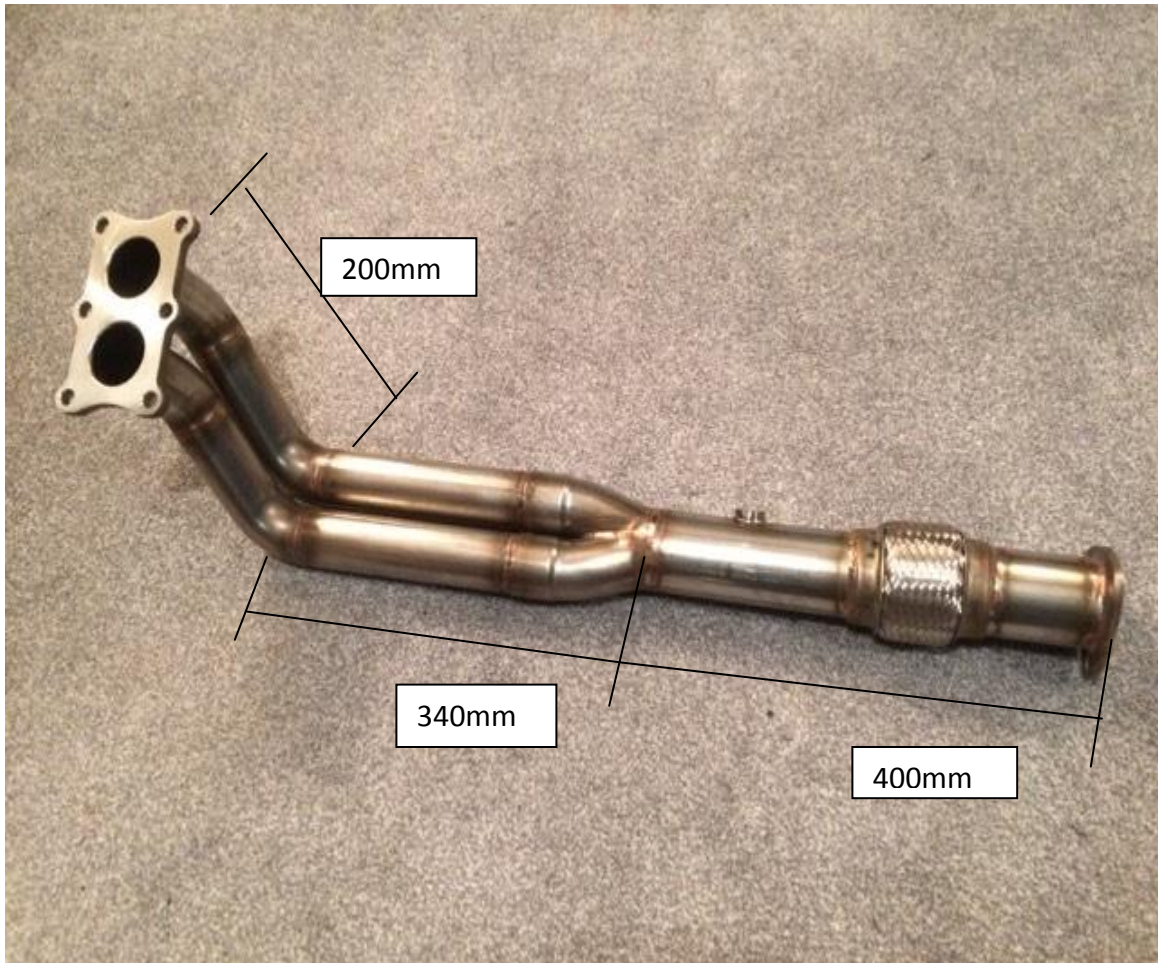
Fig 1 Downpipe (material:- mild steel or stainless steel)
